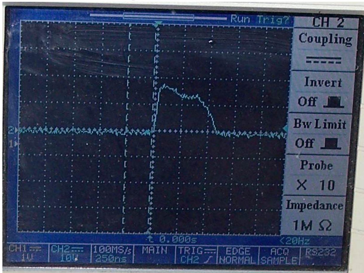
TENMA DSO RF Envelope
